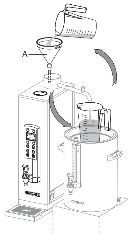
Descaling procedure
